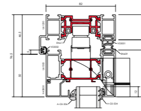
F82 Head
