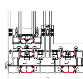
Sill Detail
